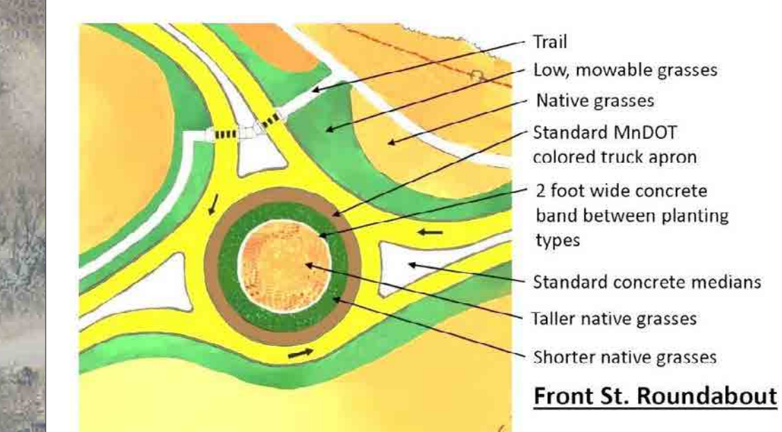
CONCRETE BAND BETWEEN PLANTINGS WITHIN ROUNDABOUT
