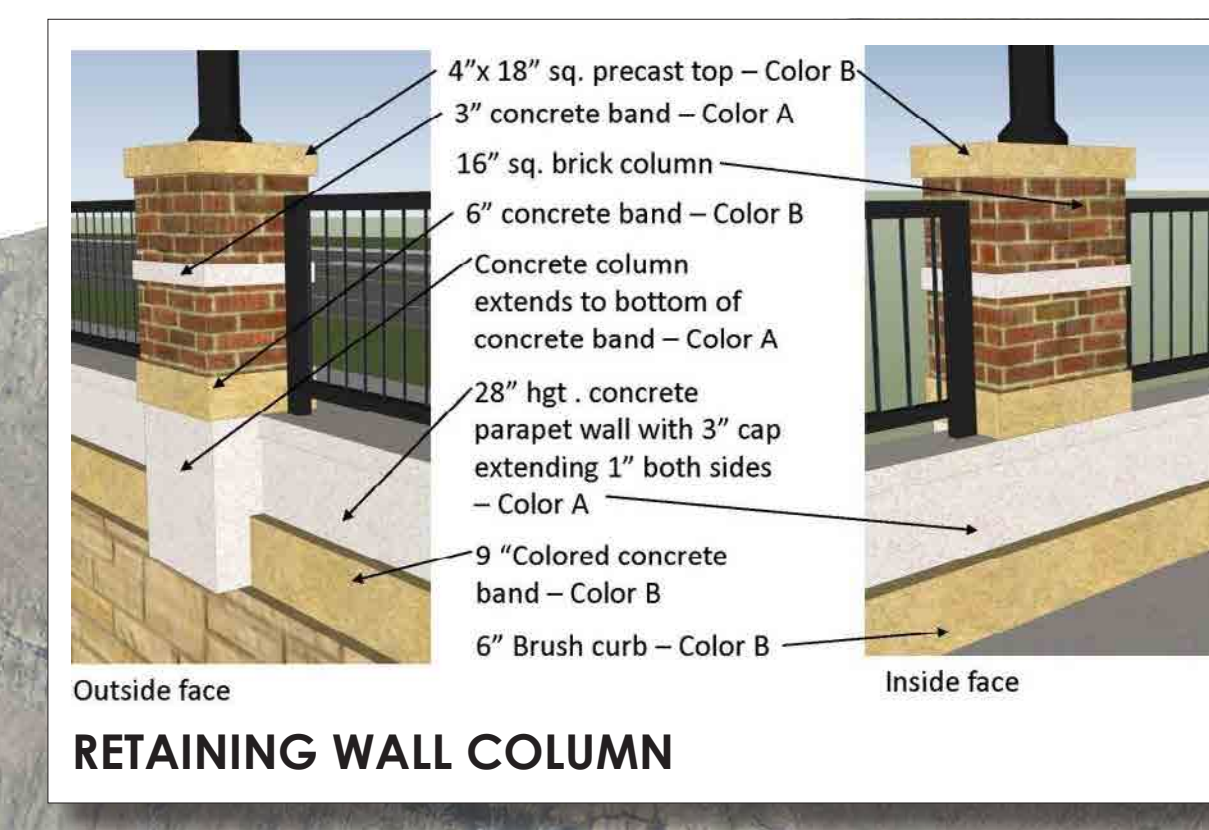
RETAINING WALL COLUMN
