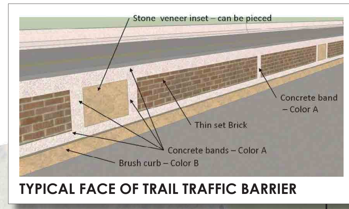
TYPICAL FACE OF TRAIL TRAFFIC BARRIER
