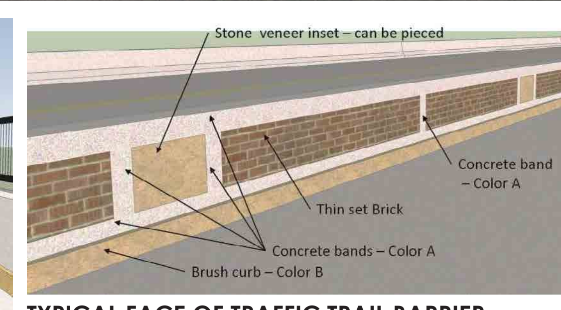
TYPICAL FACE OF TRAIL TRAFFIC BARRIER
