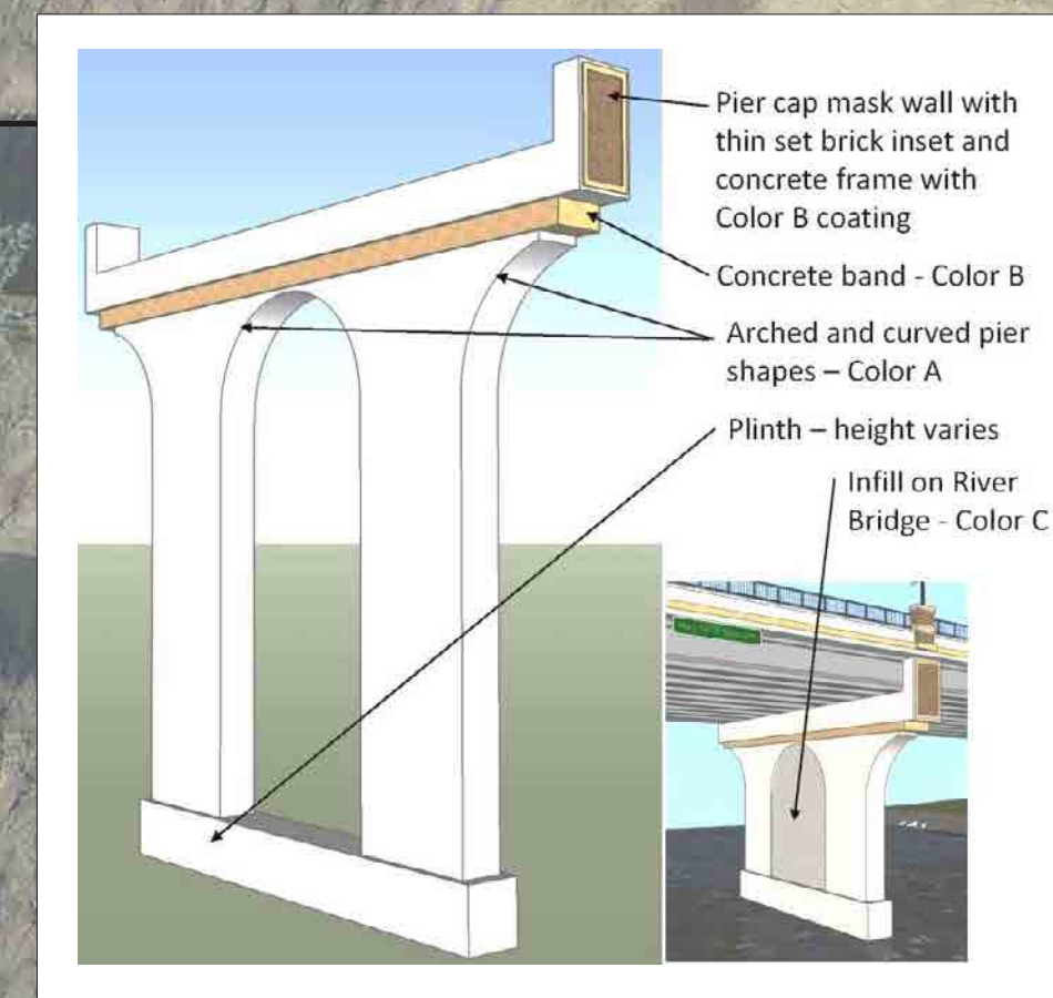
TYPICAL PIERS
