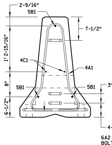
SECTION B-B TYPICAL SECTION
